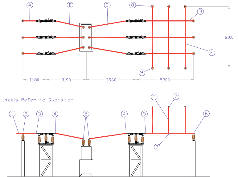
Diagram showing connector designs for substation layouts
